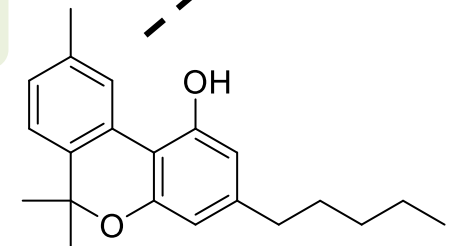
cannabinol (CBN)
