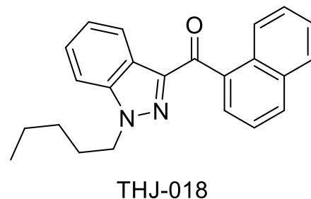
série naphthoyl-indazole
