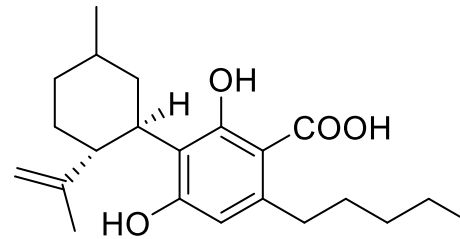
acide cannabidiolique
