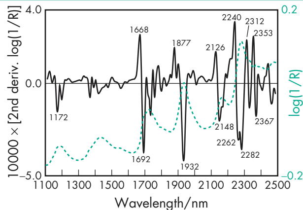
Figure 1: Near-infrared spectrum of crosopvidone measured by reflectance.
