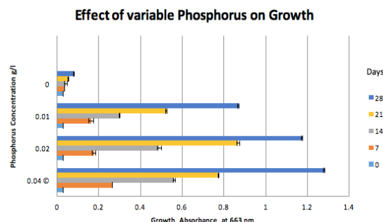
Figure 1. Effect of variable phosphorus concentration on growth of Chlorella vulgaris . (Absorbance at 663 nm; 0.04g/l is control).
