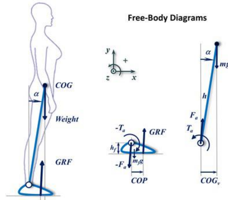
Image : « The inverted pendulum model of the human standing », Marcos Duarte, BMClab GitHub repository
